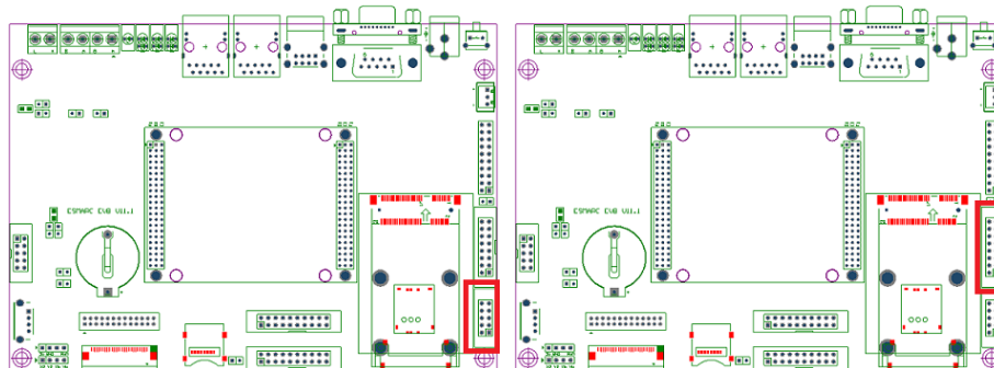
CN17:U_JTAG_(xxx)端口
